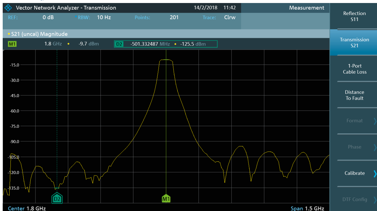
R&S®FPC1500 S_{21} scalar transmission measurement with the R&S®FPC-K42 option
